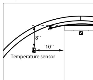
Barrel Sauna Temperature Sensor Location
