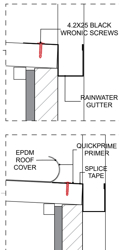
ILLUSTRATIVE DRAWING OF THE INSTALLATION PRINCIPLE
