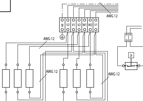
Mythos S35 internal wiring single-circuit
