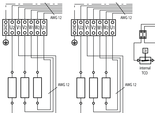
Mythos S35 internal wiring dual-circuit
